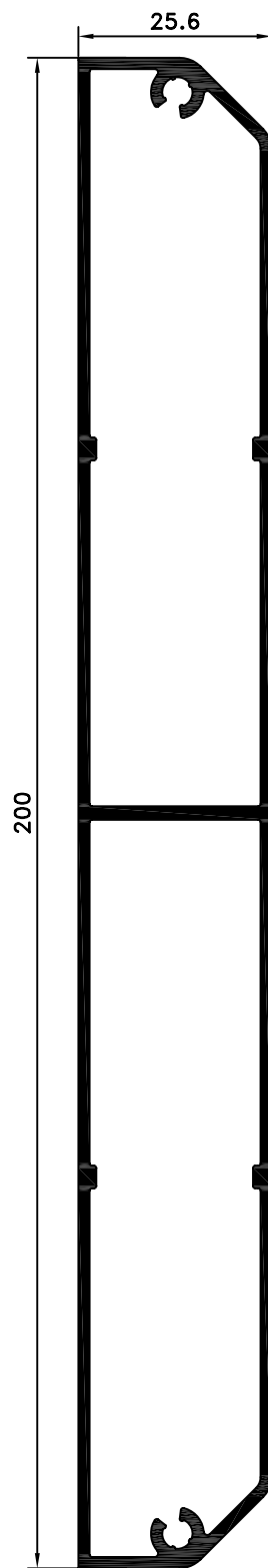
REF. 11031 Lama tablón biselada 200x25,6mm APT 031
