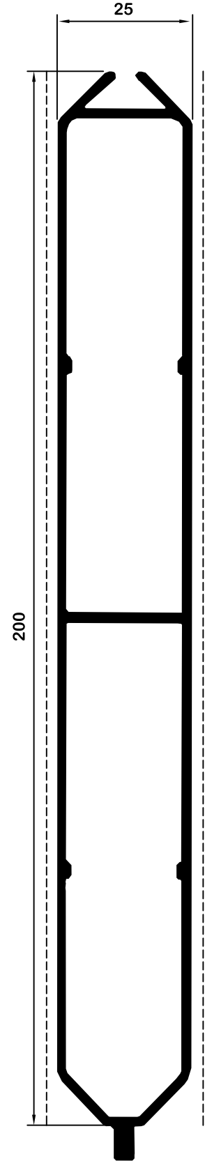
REF. 11035 Lama biselada simétrica 200x25 TPT 035
