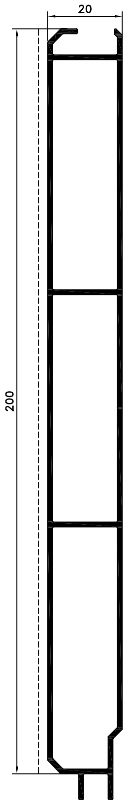
REF. 11030 Lama 200x20 c/ bisel APT 030
