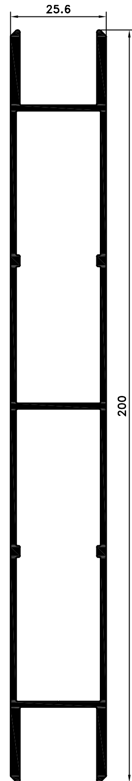
REF. 11032 Lama 200x25,6 p/ tubo 20mm APT 032
