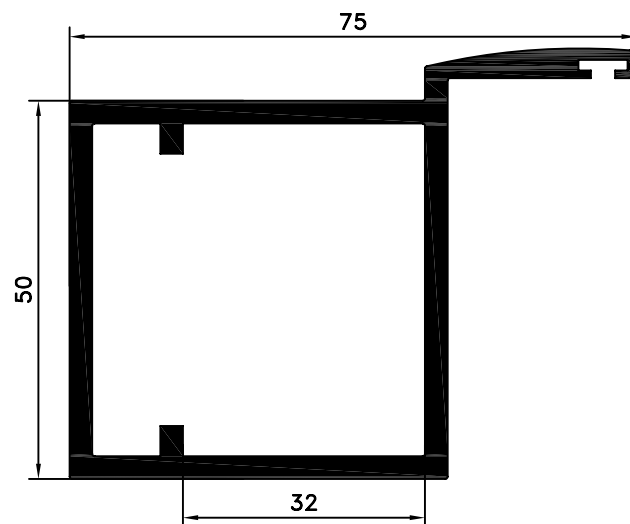
REF. 110002 Marco TPT 02
