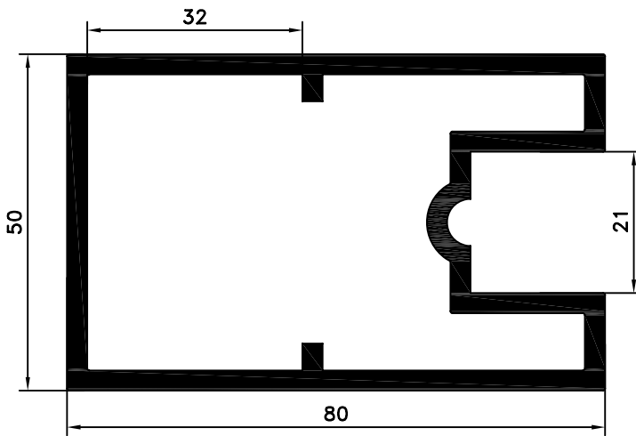
REF. 110003 Hoja lama 20 mm TPT 03
