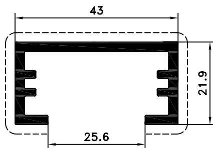
REF. 11007 Perfil U APT 007
