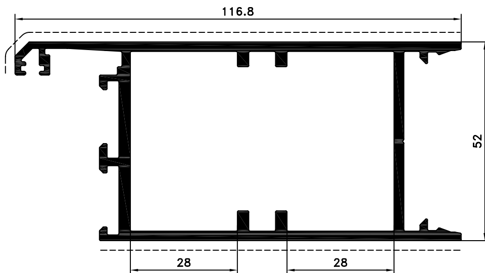
REF. 11002 Hoja grande APT 002
