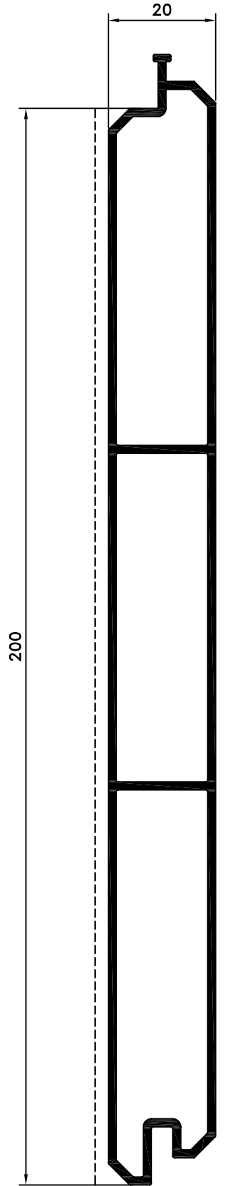
REF. 11020020 Lama biselada 200x20 TPT 09
